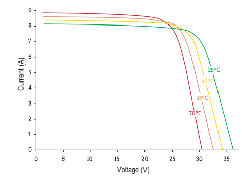
SLK60P6L - 225W I-V characteristics with a variety of cell temperatures at 92.94 W/ft² (1,000 W/m²)
